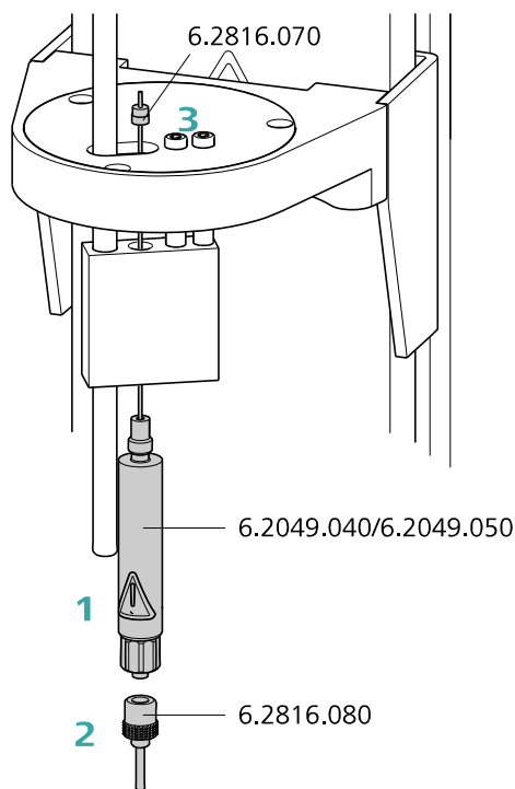
Figure 5 Mounting the needles
