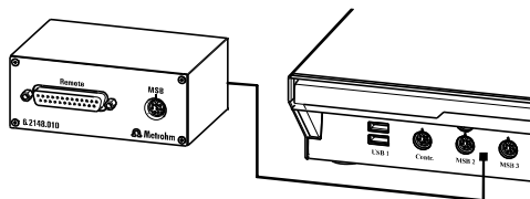
Figure 22 Connecting the Remote Box
