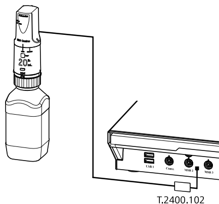
Figure 19 Connecting a dosing device
