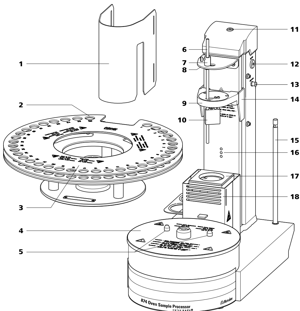
Figure 1 Front 874 Oven Sample Processor
