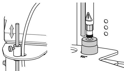
Figure 16 Adjusting the guide rod
