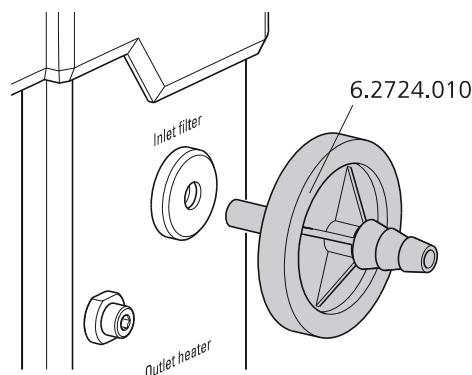
Figure 10 Mounting the dust filter
