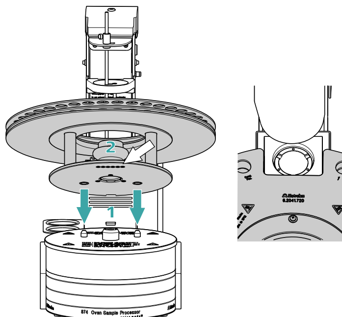
Figure 15 Attaching rack
