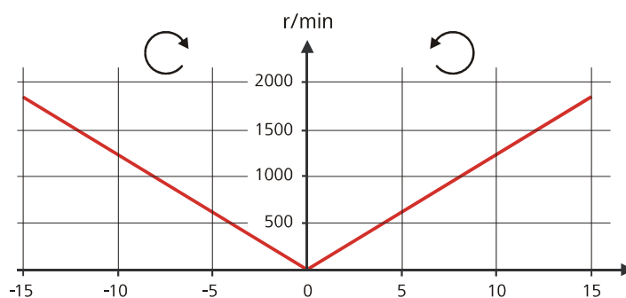
Figure 26 Rotational speed depending on the stirring rate
