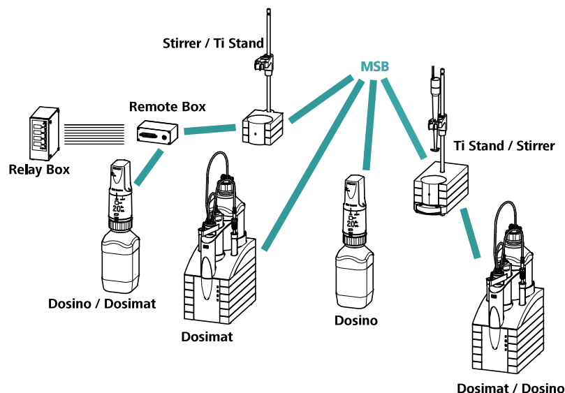
Figure 18 MSB connections
