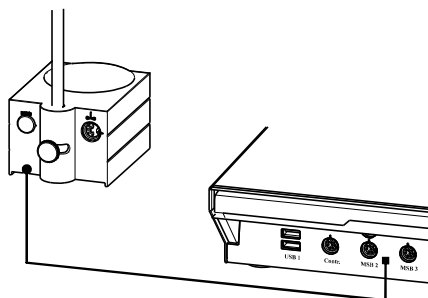
Figure 20 Connecting an MSB stirrer
