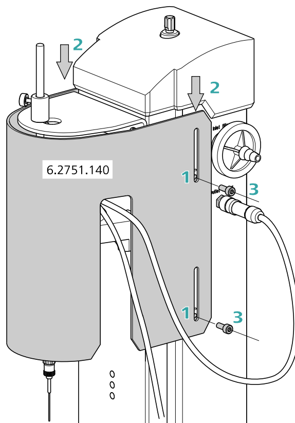
Figure 12 Mounting the safety shield
