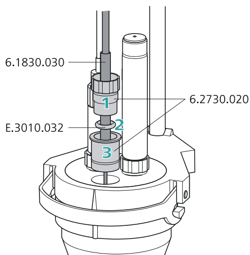
Figure 14 Volumetric KF titration cell
