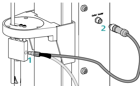
Figure 7 Mounting the heating tubing
