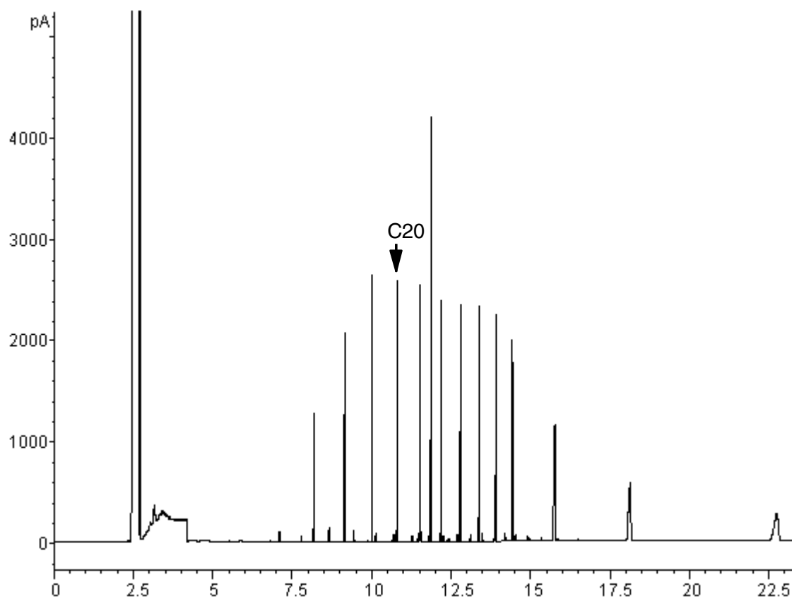
Figure 64 Chromatogram from ten 10 \mu L injections
