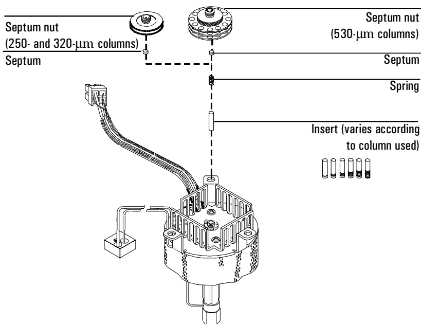
Figure 54 The cool on-column inlet for automatic injection systems
