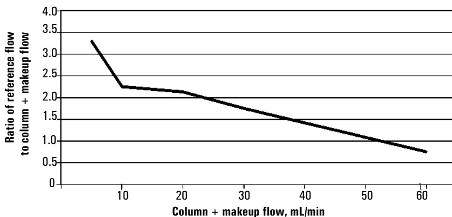
Figure 78. Selecting the reference gas flow
