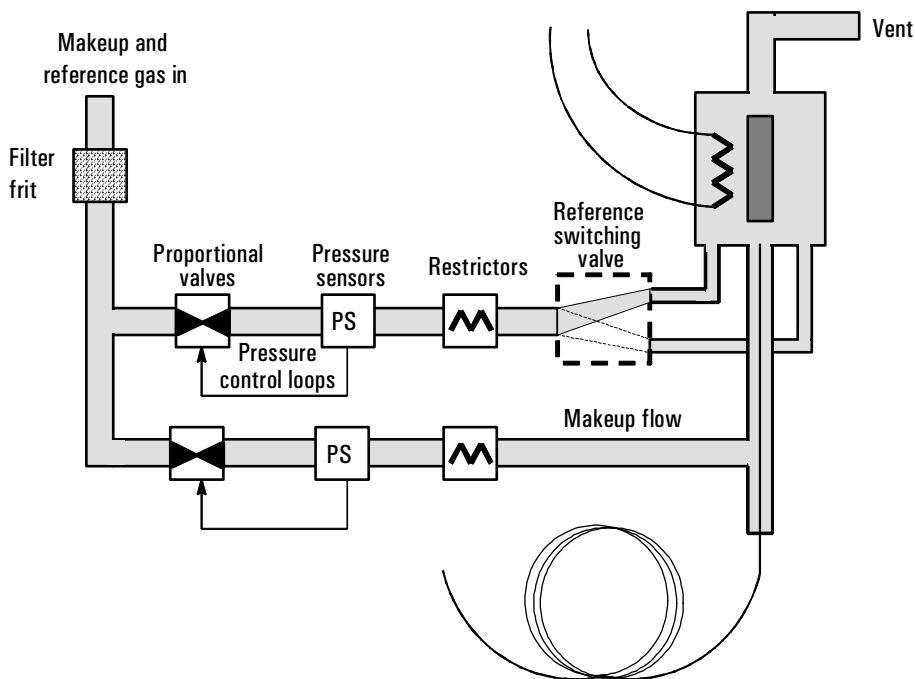
Figure 77. TCD pneumatics
