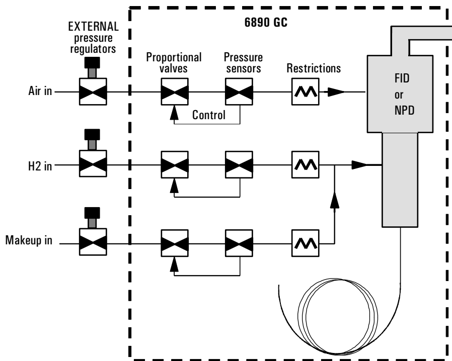
Figure 7 Internal/external plumbing: FID and NPD with EPC
