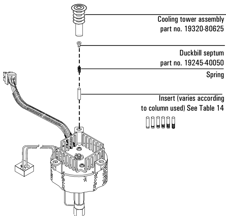
Figure 55 The cool on-column inlet for manual injection systems
