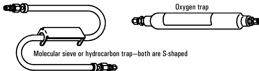
Figure 96. Traps
