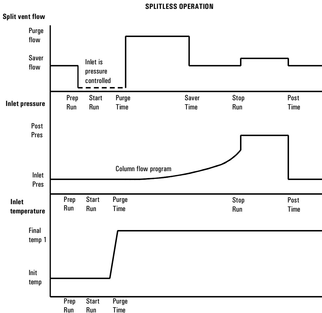
Figure 61 Flows, pressures, and temperatures
