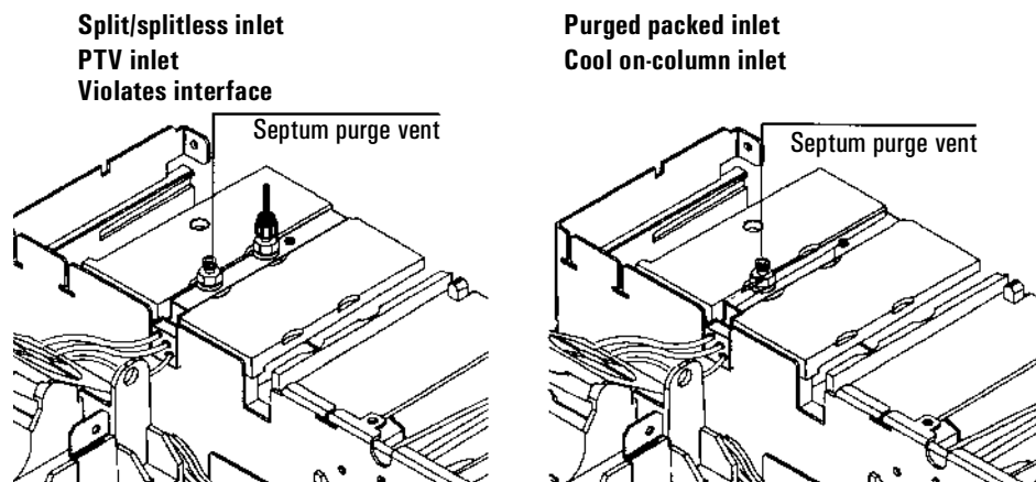
Figure 41 Septum purge vents
