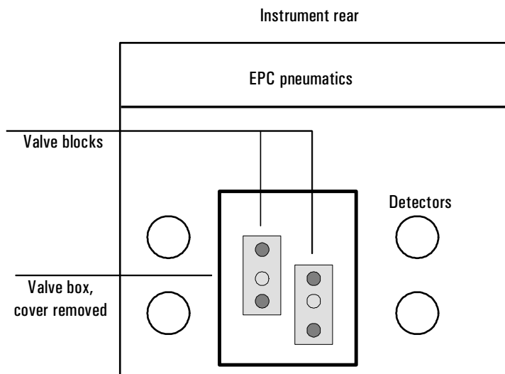
Figure 28 The valve box
