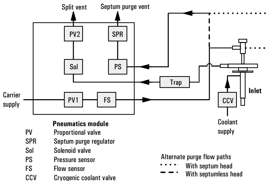
Figure 56 PTV system components
