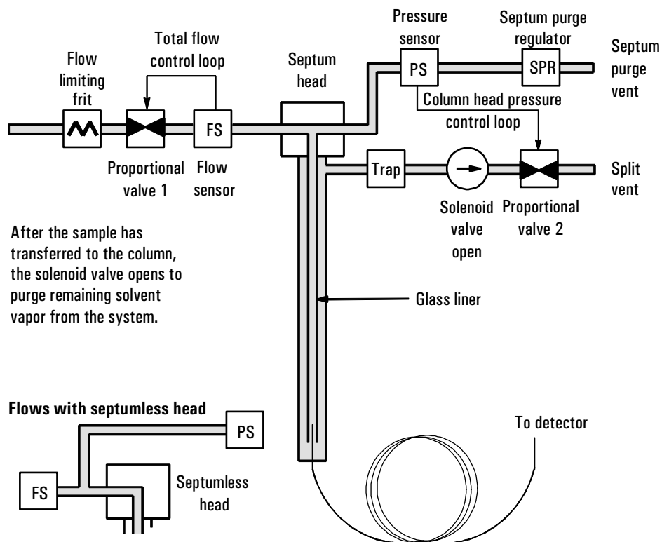
Figure 60 Stage 2. Purging
