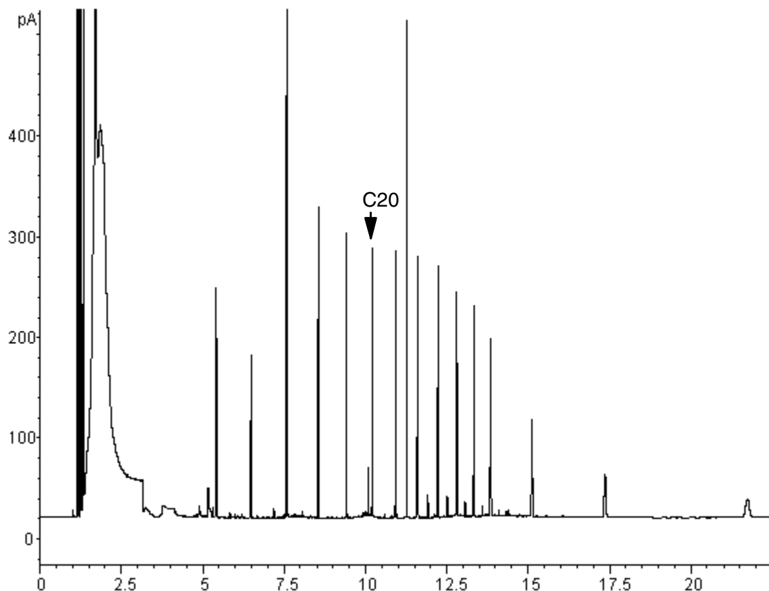
Figure 63 Chromatogram from one 10 \mu L injection
