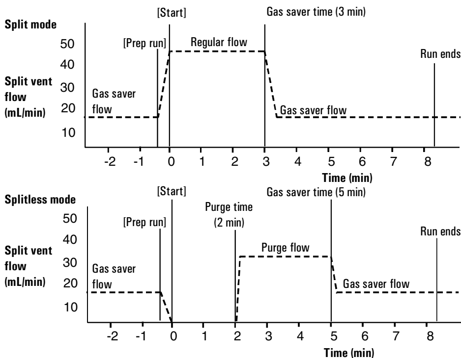
Figure 40 Gas saver operation
