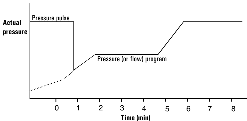
Figure 58 Pressure pulse and column flow or pressure
