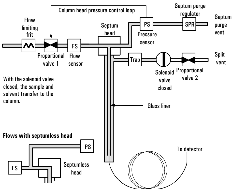
Figure 59 Stage 1. Sample injection
