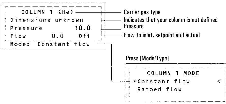
Figure 39 Column display — Packed or undefined capillary columns
