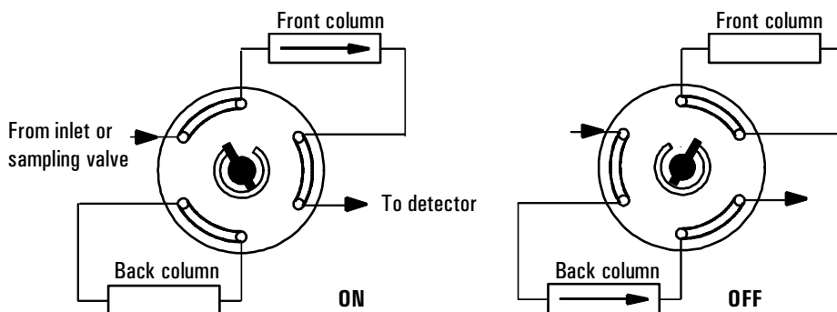
Figure 31 A column selection valve
