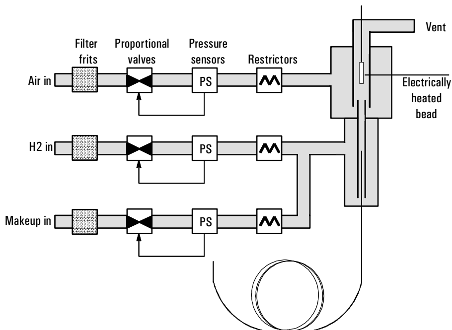
Figure 82. NPD pneumatics
