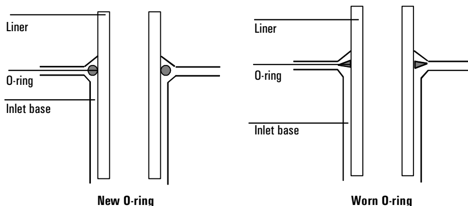
Figure 47 Cross section of inlet, liner, and O-ring
