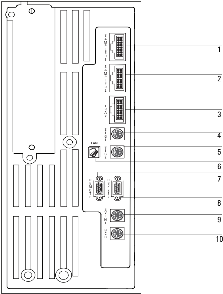
Figure 111. Overview of cable connections on the back of the GC
