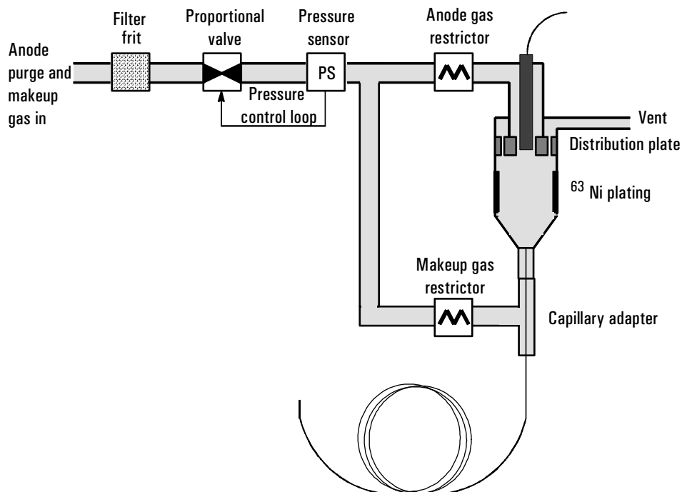
Figure 87. μ-ECD pneumatics
