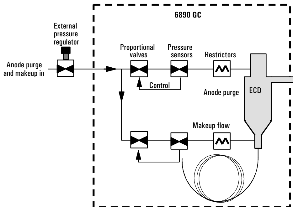
Figure 9 Internal/external plumbing: ECD with EPC
