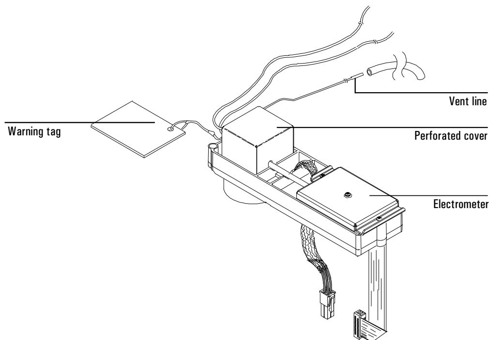
Figure 89. The \mu -ECD
