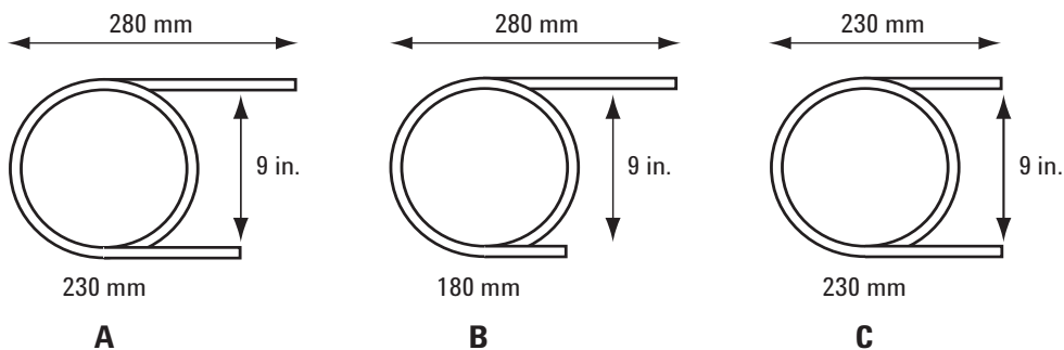
Figure 19. Column Configurations
