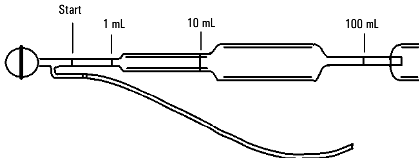
Figure 12 A three-volume bubble meter
