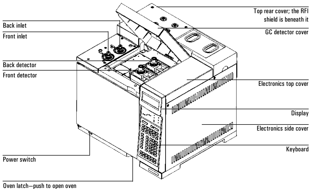
Figure 98. Front view of GC
