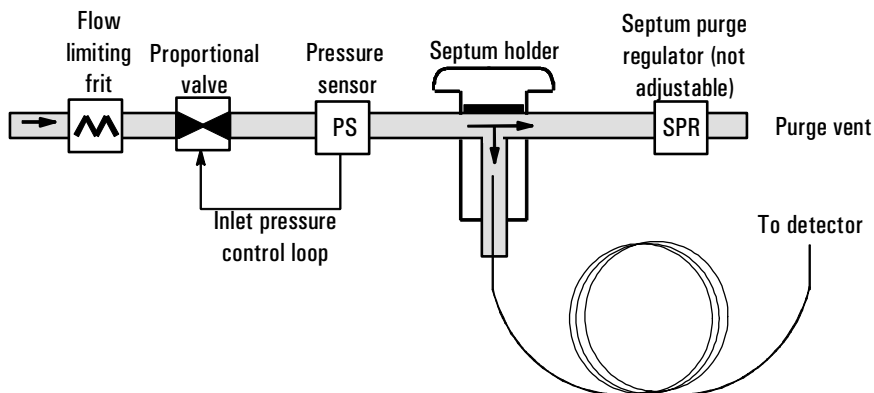
Figure 52 Cool on-column capillary inlet with EPC
