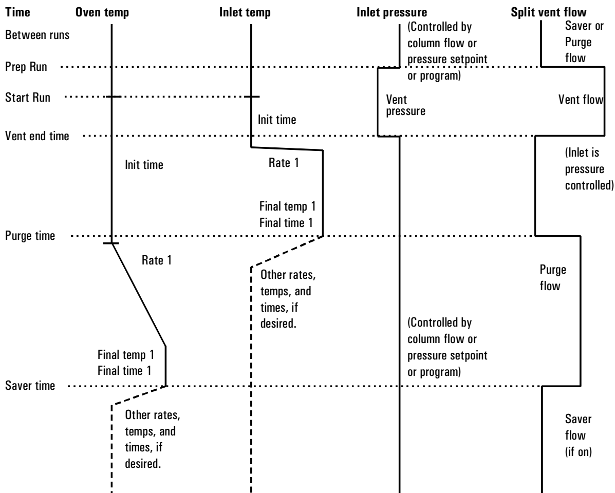
Figure 62 Time relationships
